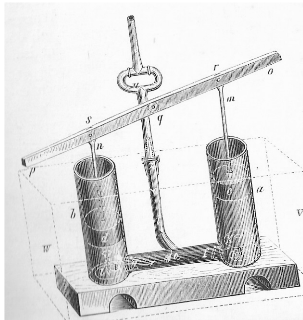
Heronova brizgalna
